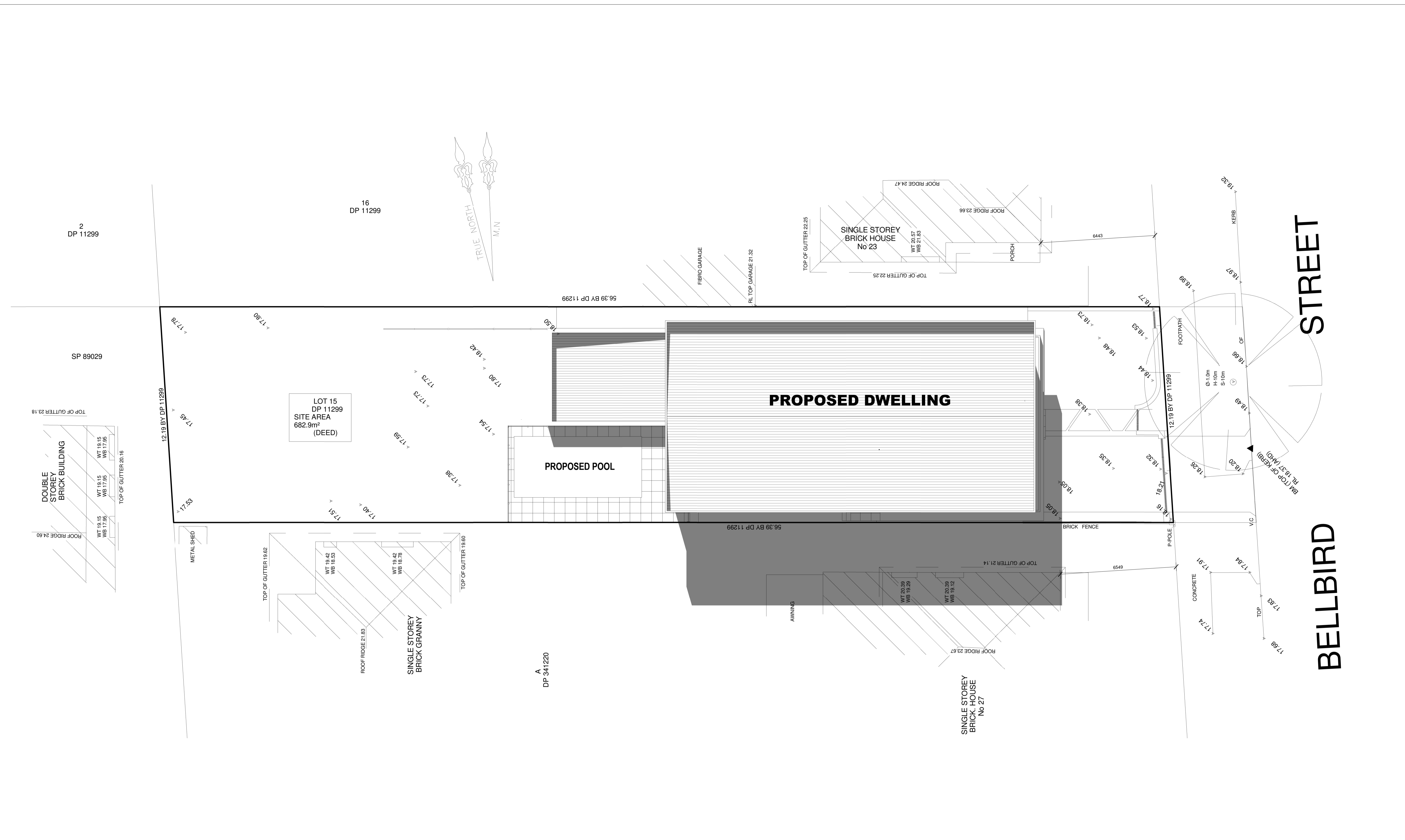
1 12PM SHADOW DIAGRAM - 21 JUNE SCALE 1:100
